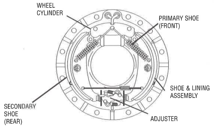
SHOE-TYPE BRAKE ASSEMBLY
