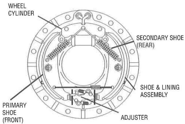
SHOE-TYPE BRAKE ASSEMBLY
